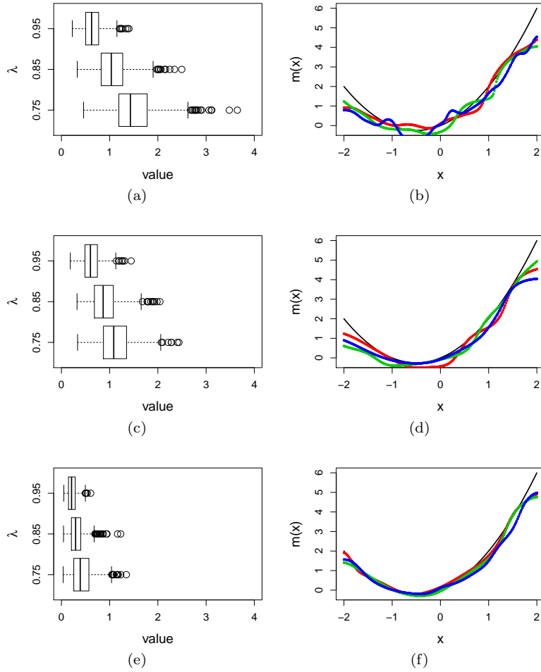
FIG H.1. Results under (C1) using approximated theoretical optimal bandwidths. Panels (a), (c), and (e): boxplots of ISEs versus \lambda for \hat{M}_N(x) , \hat{M}_0(x) , and \hat{M}_1(x) , respectively. Panels (b), (d), and (f): estimated mode curves, \hat{M}_N(x) , \hat{M}_0(x) , and \hat{M}_1(x) , respectively, when \lambda = 0.85 . In each panel with estimated mode curves associated with an estimator, the black line depicts the true mode curve, the red, green, and blue lines are three estimated mode curves from the same method that yield ISE being the first, second, and third quantiles among the 500 ISEs for that method from the simulation, respectively.
