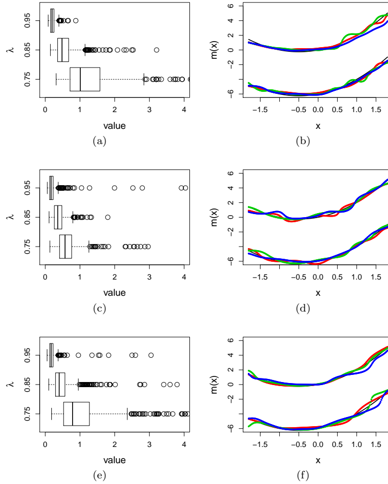
FIG H.4. Results under (C2) using the CV-SIMEX bandwidth selection. Panels (a), (c), and (e): boxplots of ISEs versus \lambda for \hat{M}_N(x) , \hat{M}_0(x) , and \hat{M}_1(x) , respectively. Panels (b), (d), and (f): estimated mode curves, \hat{M}_N(x) , \hat{M}_0(x) , and \hat{M}_1(x) , respectively, when \lambda = 0.85 . In each panel with estimated mode curves associated with an estimator, the black lines depict the true mode curves, the red, green, and blue lines are three estimated mode curves from the same method that yield ISE being the first, second, and third quantiles among the 500 ISEs for that method from the simulation, respectively.
