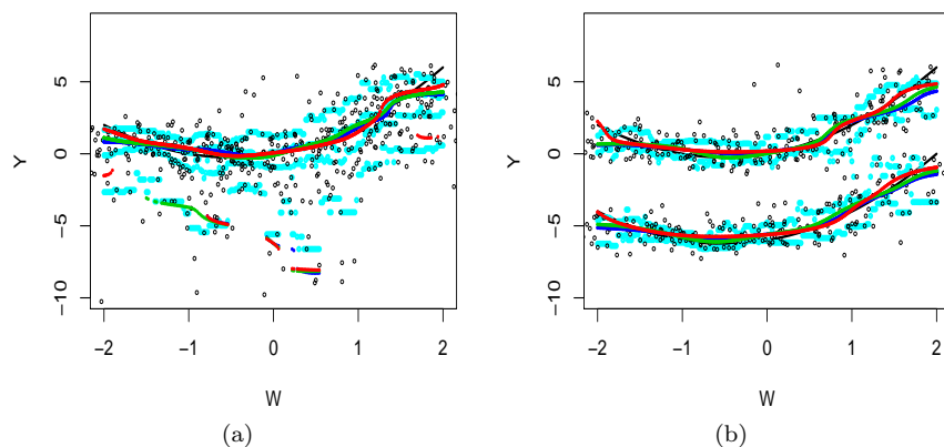
FIG 1. Estimated mode curves using one data set generated from each of (C1) (panel (a)) and (C2) (panel (b)), incorporating the data-driven bandwidth selection and data-dependent starting values (in turquoise). Each panel contains the truth M(x) (black lines), \hat{M}_N(x) (blue lines), \hat{M}_0(x) (green lines), and \hat{M}_1(x) (red lines).
