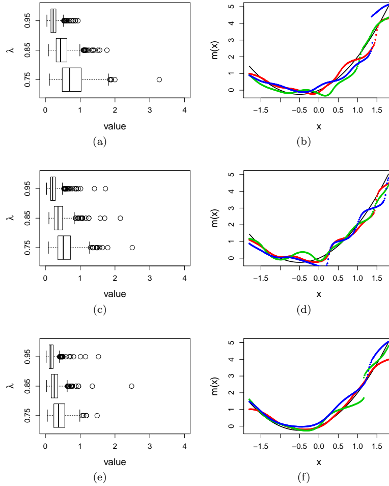
FIG H.3. Results under (C1) using the CV-SIMEX bandwidth selection. Panels (a), (c), and (e): boxplots of ISEs versus \lambda for \hat{M}_N(x) , \hat{M}_0(x) , and \hat{M}_1(x) , respectively. Panels (b), (d), and (f): estimated mode curves, \hat{M}_N(x) , \hat{M}_0(x) , and \hat{M}_1(x) , respectively, when \lambda = 0.85 . In each panel with estimated mode curves associated with an estimator, the black line depicts the true mode curve, the red, green, and blue lines are three estimated mode curves from the same method that yield ISE being the first, second, and third quantiles among the 500 ISEs for that method from the simulation, respectively.
