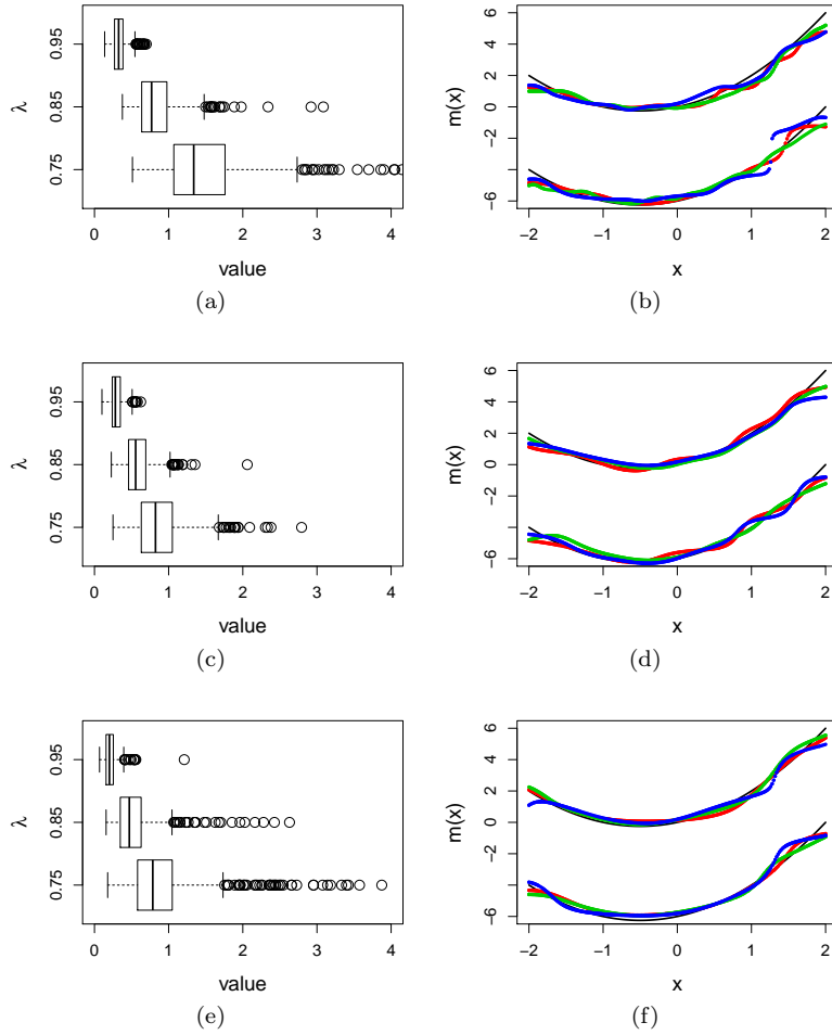
FIG H.2. Results under (C2) using approximated theoretical optimal bandwidths. Panels (a), (c), and (e): boxplots of ISEs versus \lambda for \hat{M}_N(x) , \hat{M}_0(x) , and \hat{M}_1(x) , respectively. Panels (b), (d), and (f): estimated mode curves, \hat{M}_N(x) , \hat{M}_0(x) , and \hat{M}_1(x) , respectively, when \lambda = 0.85 . In each panel with estimated mode curves associated with an estimator, the black lines depict the true mode curves, the red, green, and blue lines are three estimated mode curves from the same method that yield ISE being the first, second, and third quantiles among the 500 ISEs for that method from the simulation, respectively.
