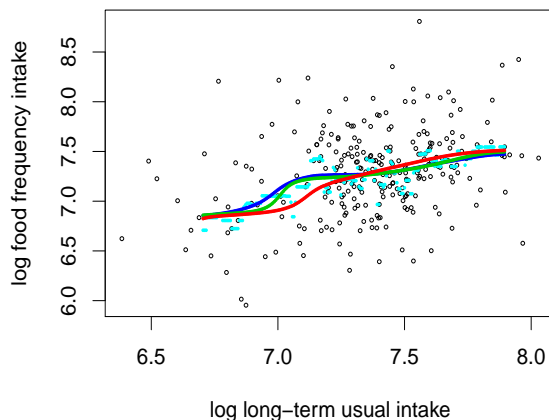
FIG 2. The dietary data (black circles) and three estimated mode curves: the naive estimate \hat{M}_N(x) (blue line), and our proposed estimates accounting for measurement error, \hat{M}_0(x) (green line) and \hat{M}_1(x) (red line). Turquoise points are the data-dependent starting values for the mean-shift algorithm.
