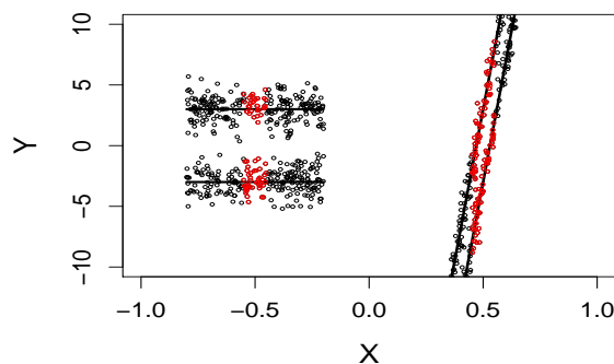
FIG 3. Illustration of two pairs of mode curves, one pair being steeper than the other pair as functions of x . The red data points fall within a window of width 0.1 in the x -direction centering at x = -0.5 for the left pair of curves and x = 0.5 for the right pair of curves.
